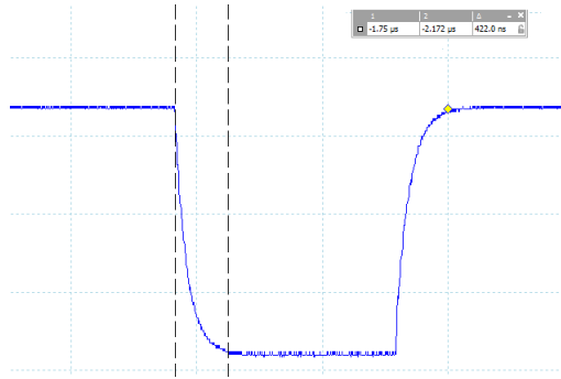
Figure 4.5: Trigger delay measurement
