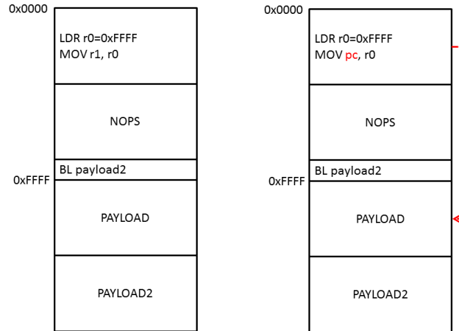
Figure 4.6: Schematic representation of the code behaviour when successfully glitched. (Left: code in normal usage, Right: code affected by the glitch)
