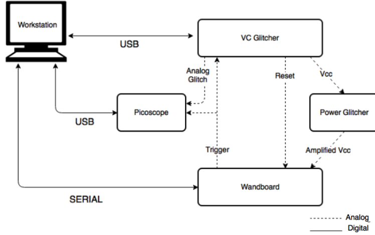
Figure 4.1: Schematic overview of the test environment
