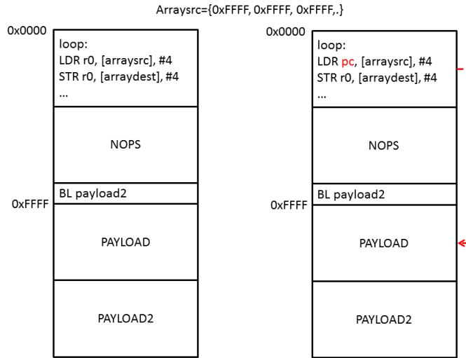
Figure 4.8: Schematic representation of the LDR corruption behaviour when successfully glitched. (Left: code in normal usage, Right: code affected by the glitch)
