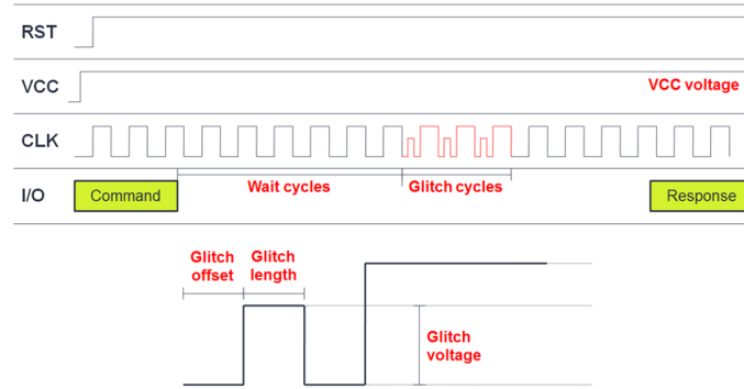
Figure 4.2: Representation of the glitch parameters needed to perform a power fault injection
