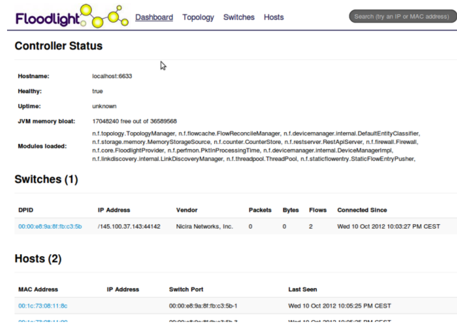
Figure 3: A Screenshot of the Floodlight web interface
