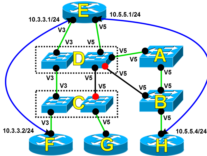
Figure 9: Complete topology
