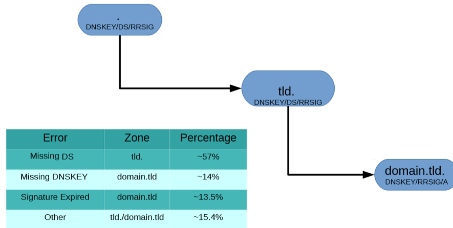
Figure I9: Misconfiguration errors
