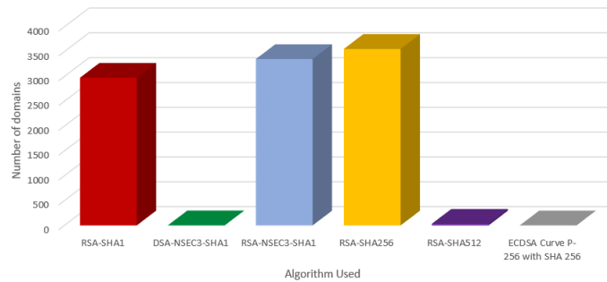
Figure 15: Algorithm
