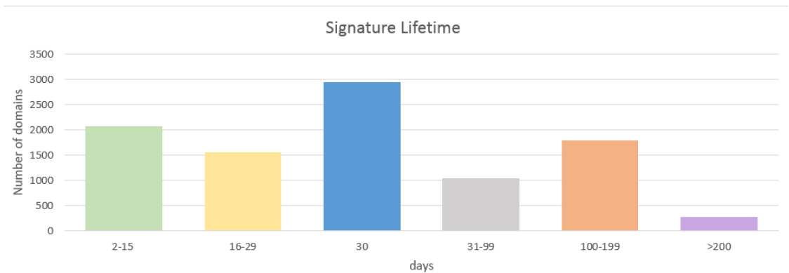
Figure 17: Signature lifetime
