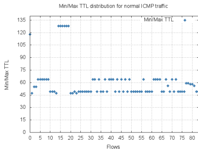
Regular ICMP
