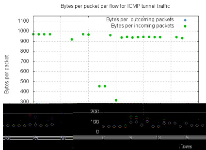
ICMP tunnel
