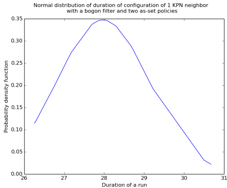
Figure 32: 1 KPN neighbor + import/export AS-SET policies
