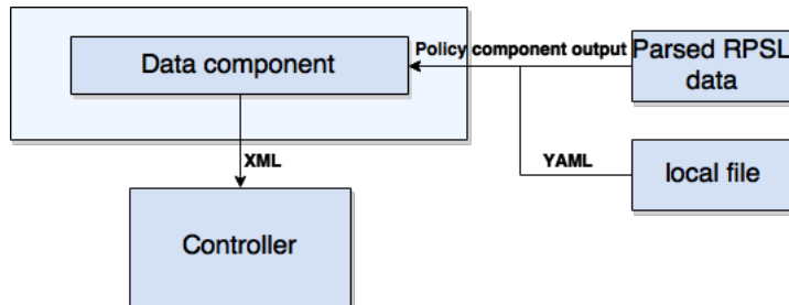
Figure 11: Policy component
