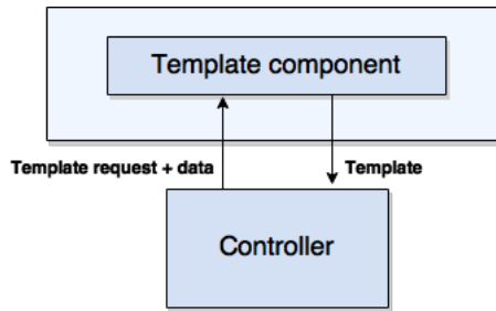
Figure 12: Template component
