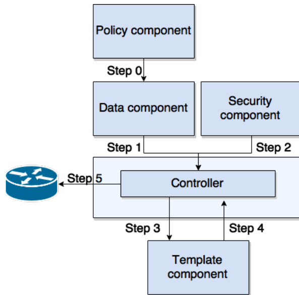
Figure 14: Controller
