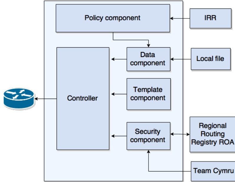
Figure 9: BGPWizard architecture
