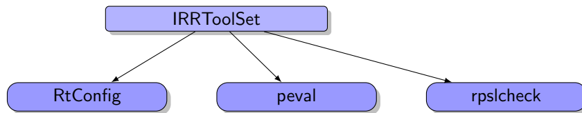
Figure 3: IRRToolSet
